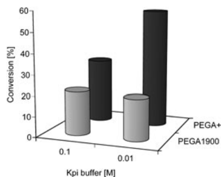
Figure 1. Comparison of the influence of polymer charge and buffer concentration on the cleavage of polymer bound phenylacetic hydrazide.
