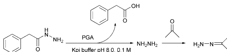
Scheme 1. Formation of hydrazine after hydrolysis by PGA and reaction with acetone with formation of hydrazone.
