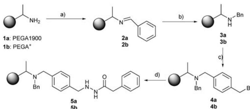
Scheme 2. a) Benzaldehyde, HC(OMe) 3 , room temperature, 24 hours; b) NaB(OAc) 3 H, MeOH, 1% AcOH (v/v), room temperature, 48 hours; c) 1,4-di(bromomethyl)benzene, DIPEA, DMF, room temperature, 48 hours; d) phenylacetic hydrazide, DMF, room temperature, 48 hours.
